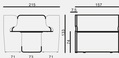
Dimensioni Workstation
