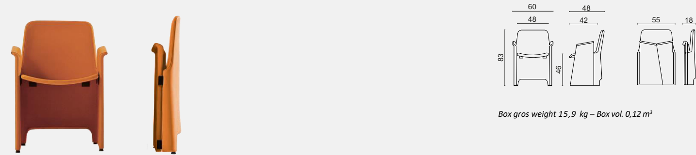
Padded folding tub armchair – mod. 1302S
